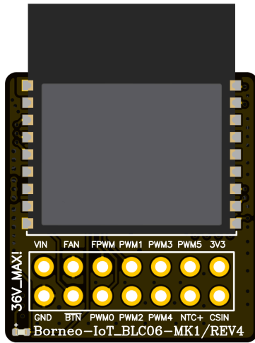
Figure 1: Appearance Diagram
